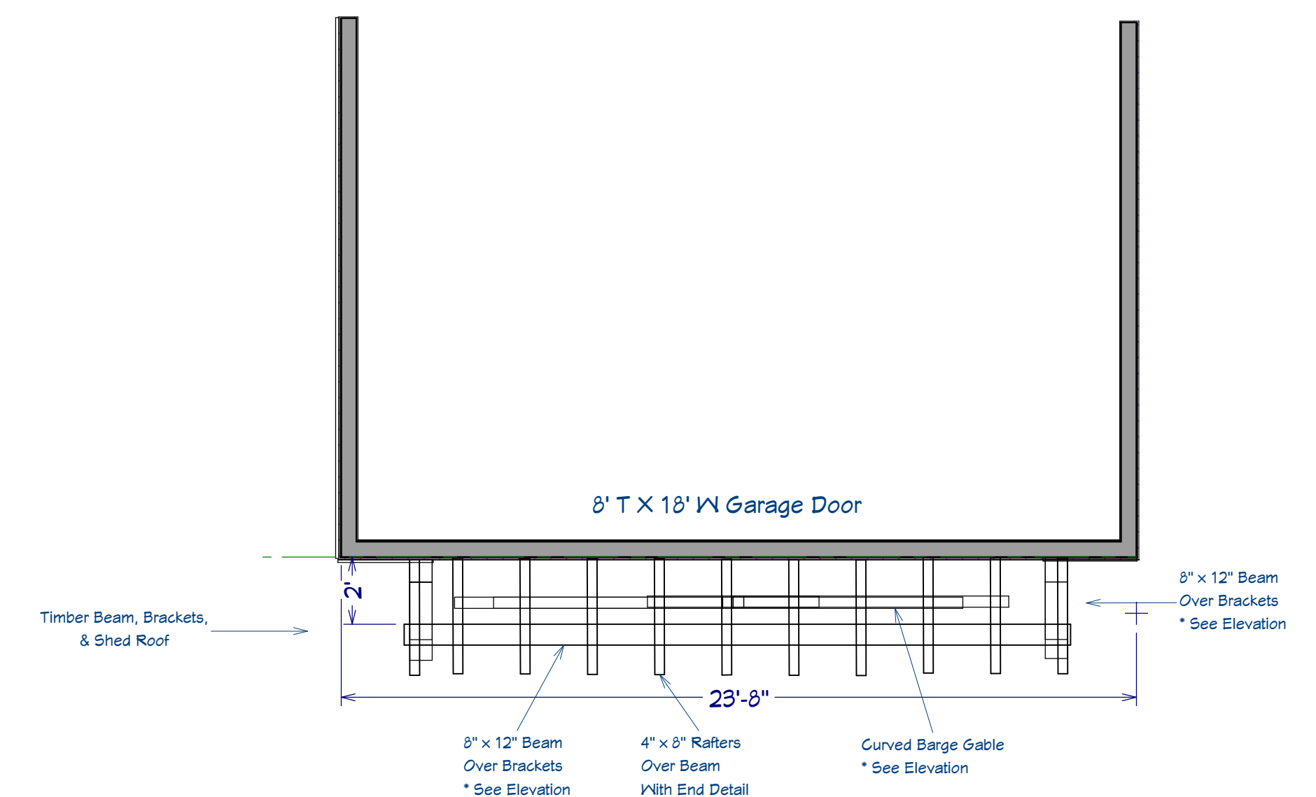
Front Porch Timbers (See Elevation)
