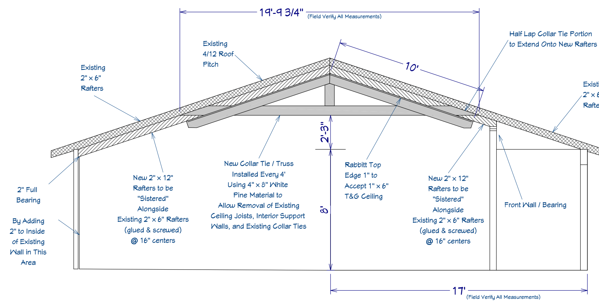
New "Sistered" 2" x 12" Rafters w/ New Timber Collar Ties
