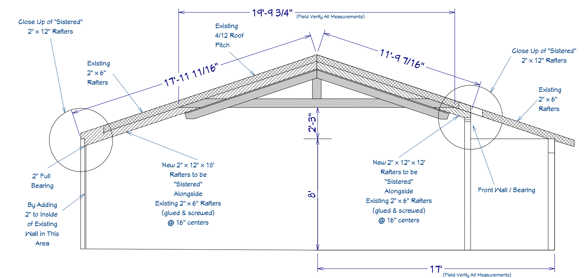
'Sistered' Rafters Bearing Closeup
