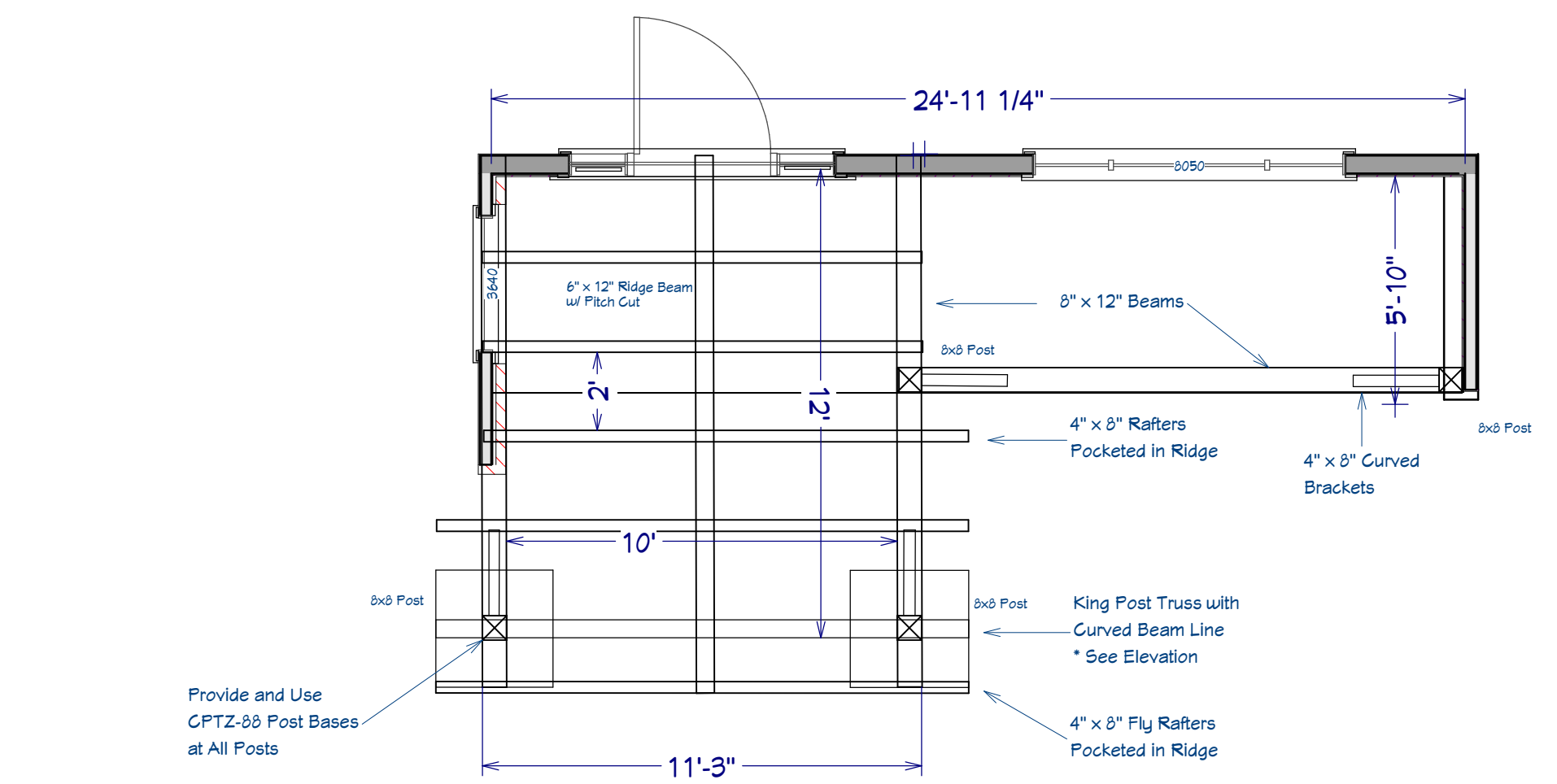
Front Porch Timbers (See Elevation)
